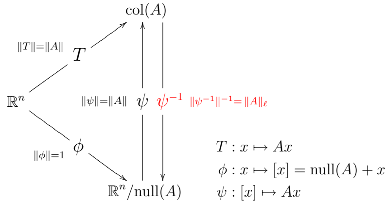
Figure 1: The commutative diagram illustrating Lemma 2.6.
